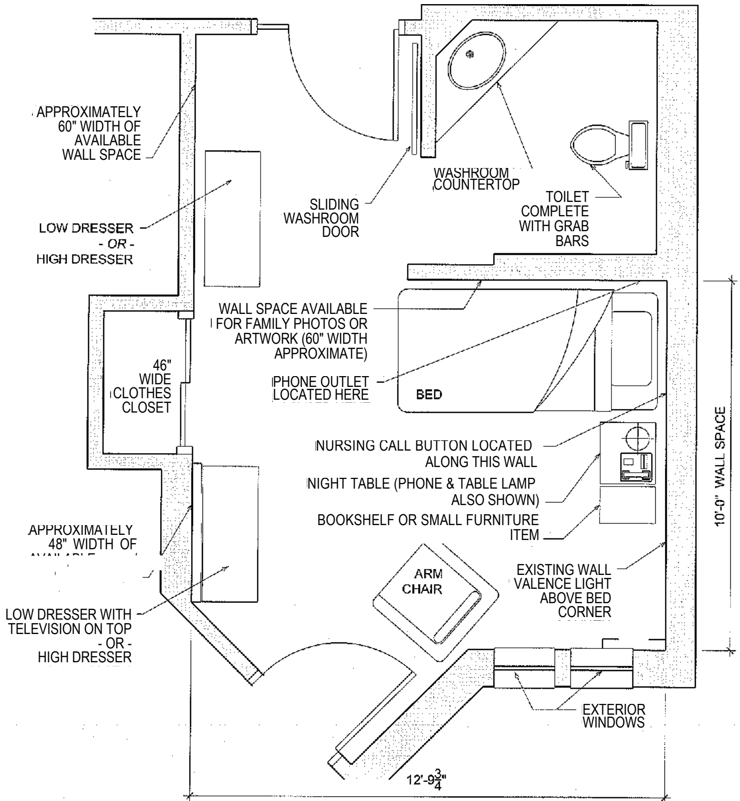
ROOM LAYOUT TYPE 'E' - LEFT-HANDED
